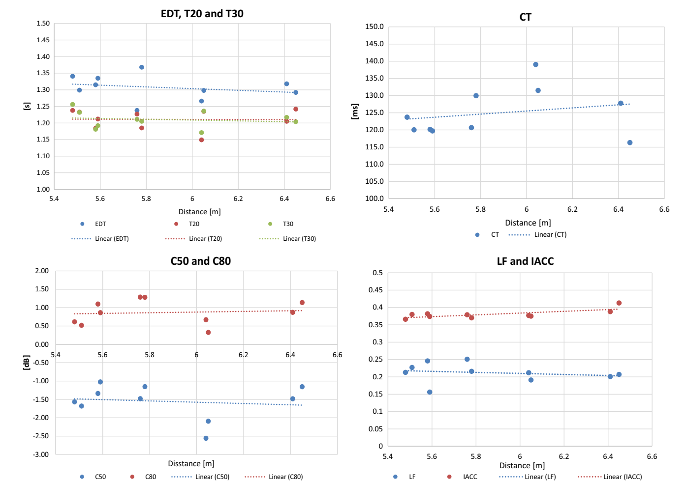
Fig. 9. Measured values of EDT, T 20 , T 30 , T s , C 50 , C 80 , LF and IACC at 1 kHz as a function of the distance from the sound source to the SoundField microphone for lateral moving.
